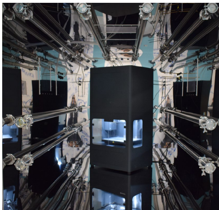
Figure 1: A 3D printer in an exposure chamber.
